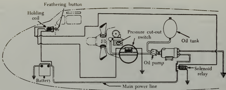
FIGURE 7-21. Typical feathering installation
